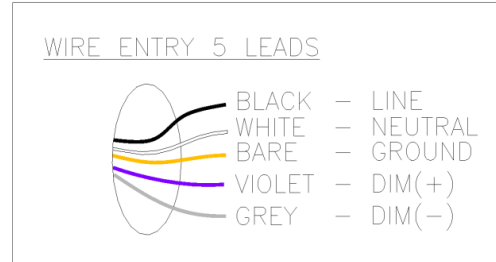
DRIVER TO LINE VOLTAGE
