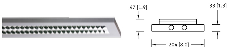
RMEC 2-T5, SL-Specular parabolic louver
